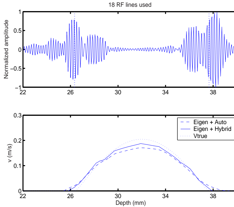
Figure 6.3. The estimated velocity profile using RF data from simulated carotid artery.
