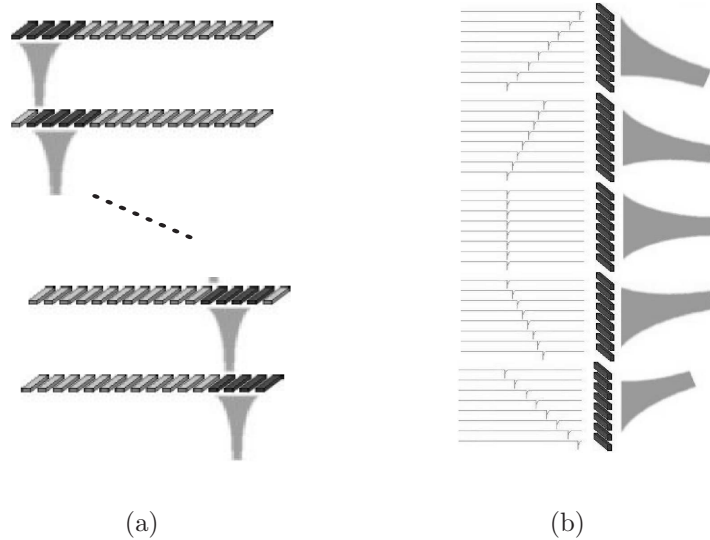
Figure 4.3. (a) A linear array transducer used to scan a medium. (b) The steering process in a phased linear array transducer.
