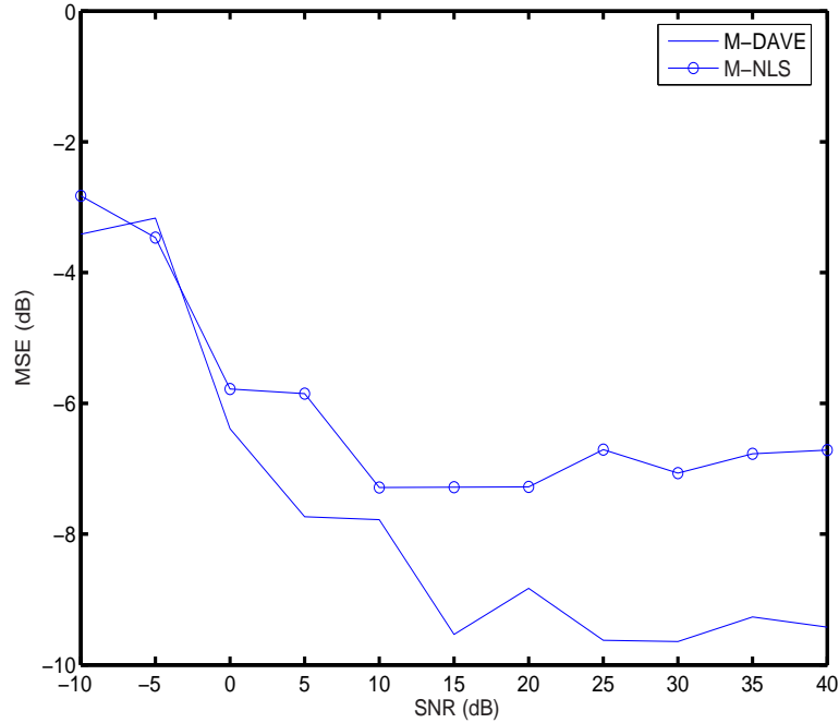
Figure 6.6. The MSE of the examined estimators as a function of the SNR, for v = 1.5 \times v_{Nyq} , with fibre flow.
