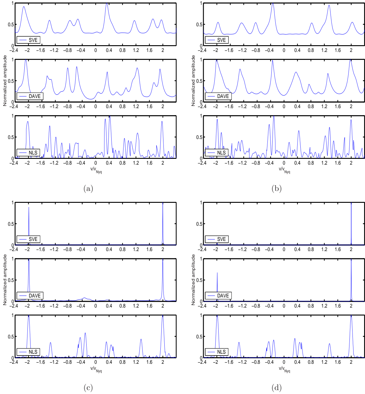
Figure 3.2. The velocity spectra using the proposed methods, with underlying true velocity, v = 2v_{Nyq} , obtained from (a) SNR = -5 dB; (b) SNR = 0 dB; (c) SNR = 10 dB; (d) SNR = 20 dB.
