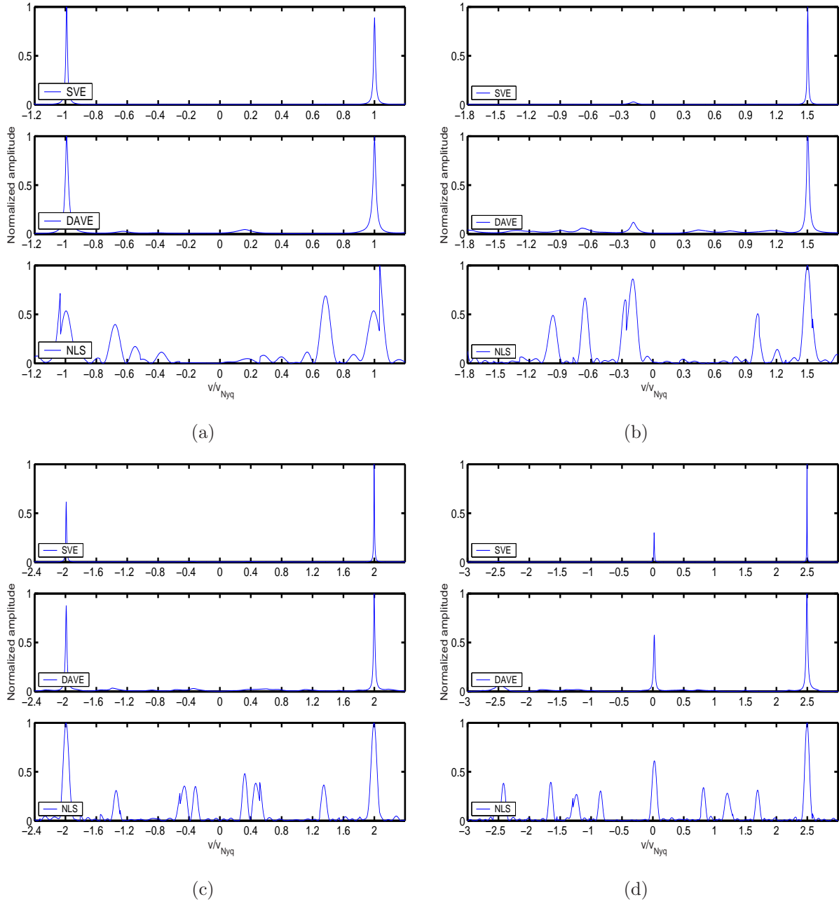
Figure 3.3. The velocity spectra using the proposed methods, with SNR = 10 dB, obtained from (a) v = v_{Nyq} ; (b) v = 1.5v_{Nyq} ; (c) v = 2v_{Nyq} ; (d) v = 2.5v_{Nyq} .
