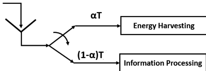
Figure 1.4: Time Switching Relaying Architecture
