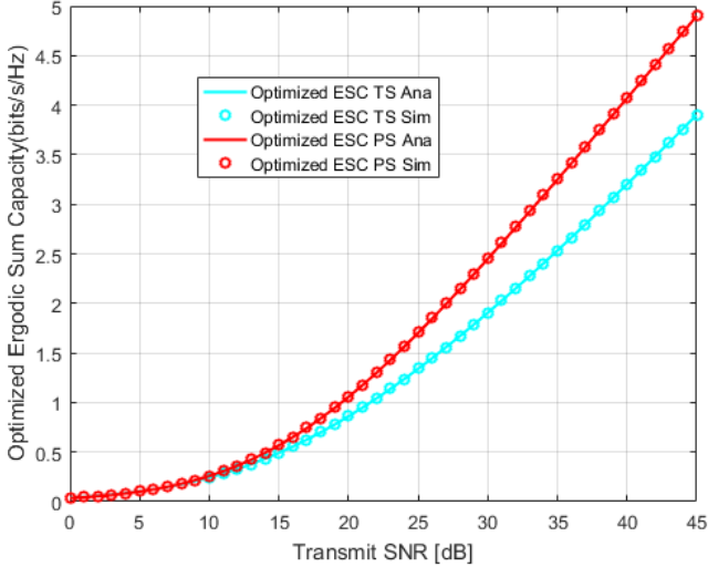
Figure 3.19: Optimized Ergodic Sum Capacity
