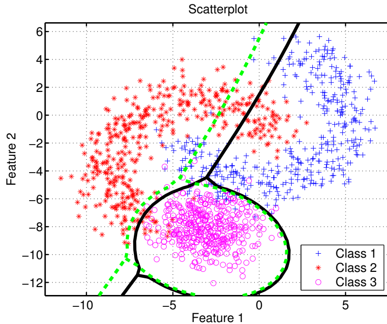
Figure 1.1: Three-class problem, illustrating a Bayes quadratic classifier at two different operating points (solid and dotted lines respectively).
