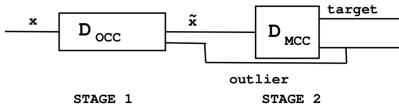
Figure 5.3: Block diagram of the SOCMC classifier. The first stage classifier D_{OCC} consists of an OCC, trained on the well defined target class. The second stage classifier D_{MCC} is a multi-class discriminant trained on examples considered to be target by the first stage.
