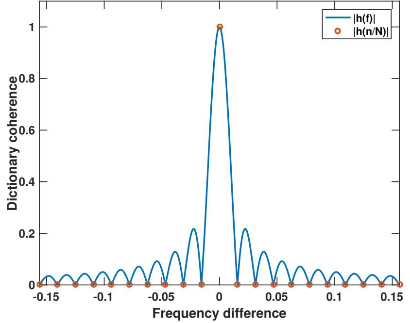
Figure 3: Absolute values of the complex function h(\Delta f) , measuring the amount of linear dependence between two Fourier vectors, spaced in frequency by \Delta f . The example illustrates the function for N = 64 samples, where orthogonality is found at every n/N , n \neq 0 .
