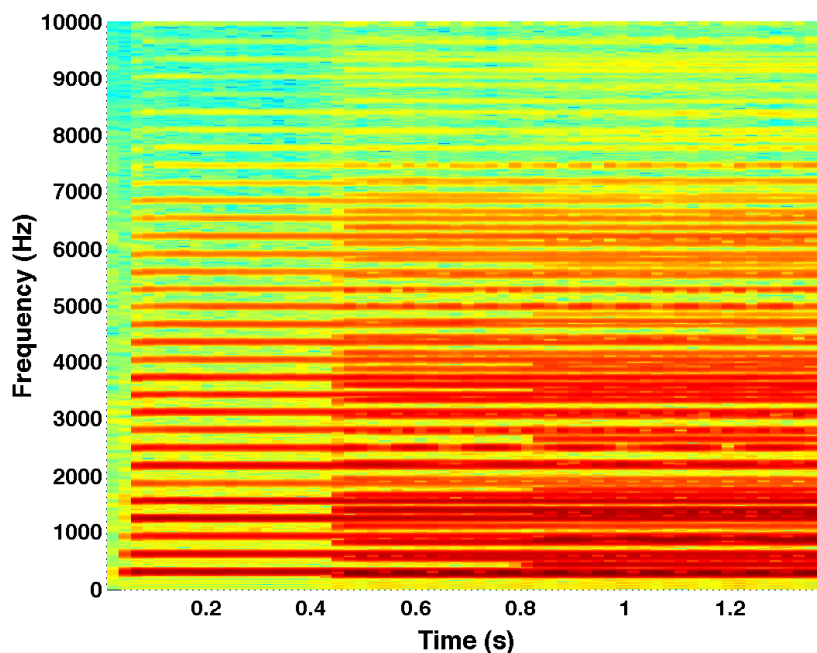
Figure 14: Spectrogram for a signal consisting of one, two and lastly three MIDI-saxophones playing notes with fundamental frequencies 311, 277, and 440 Hz, respectively.
