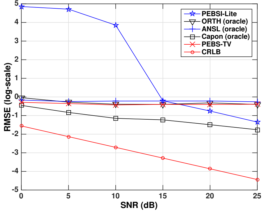
Figure 11: The RMSE for the fundamental frequency estimates for the triple pitch test signal, as compared to the (root) CRLB. For PEBSI-Lite and PEBS-TV, only estimates where the number of pitches is found are considered. For the reference methods ORTH, ANLS, Capon, and PEBS-TV only estimates where all estimated pitch frequencies lie within 2 Hz of the true pitch frequencies are considered.
