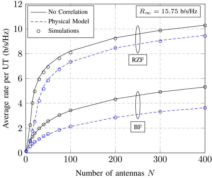
Figure 3.15: Average per-user rate versus number of antennas N for the RZF and BF precoders. Solid and dashed lines depict the asymptotic approximations, markers the simulation results.
