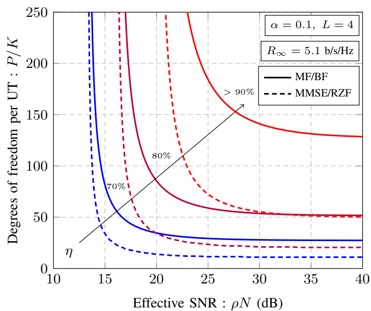
Figure 3.13: Degrees of freedom per UT P/K necessary to achieve \eta R_\infty versus effective SNR \rho N for L = 4 and \alpha = 0.1 .
