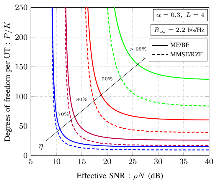
Figure 3.12: Degrees of freedom per UT P/K necessary to achieve \eta R_\infty versus effective SNR \rho N for L = 4 and \alpha = 0.3 .
