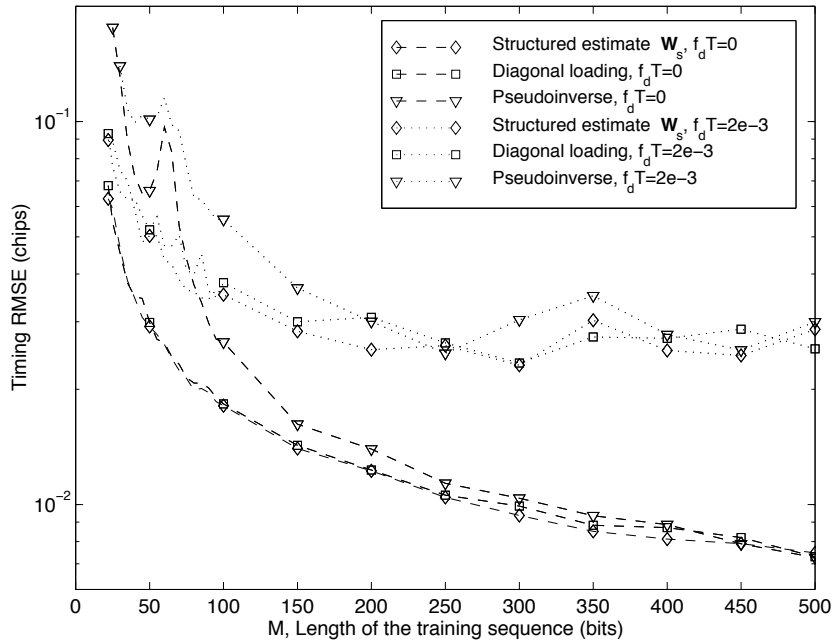
Figure 5.7: Comparison of the performance for three different estimates of the correlation matrix in two different channels. K = 10 , P = 15 , m = 4 , E_b N_0 = 4\text{dB} per antenna, \text{NFR} = 10\text{dB} , \lambda = \sigma_w^2 .
