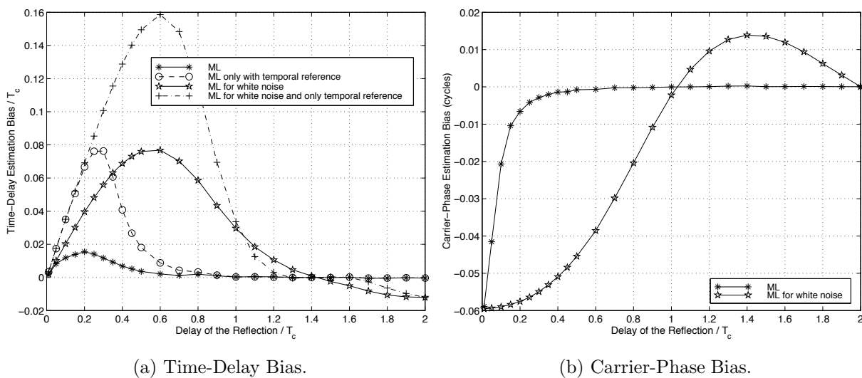
Figure 4.8: Bias of several estimators produced by a specular reflection as a function of its delay relative to the direct signal. Parameters: \check{\theta}_0 = 0^\circ , \check{\tau}_0 = 0 , \check{\theta}_1 = 10^\circ , \check{\alpha}_0 / \check{\alpha}_1 = \sqrt{2} , M = 3 pulses, m = 6 antennas, \text{SNR}_0 = 15.87 dB.
