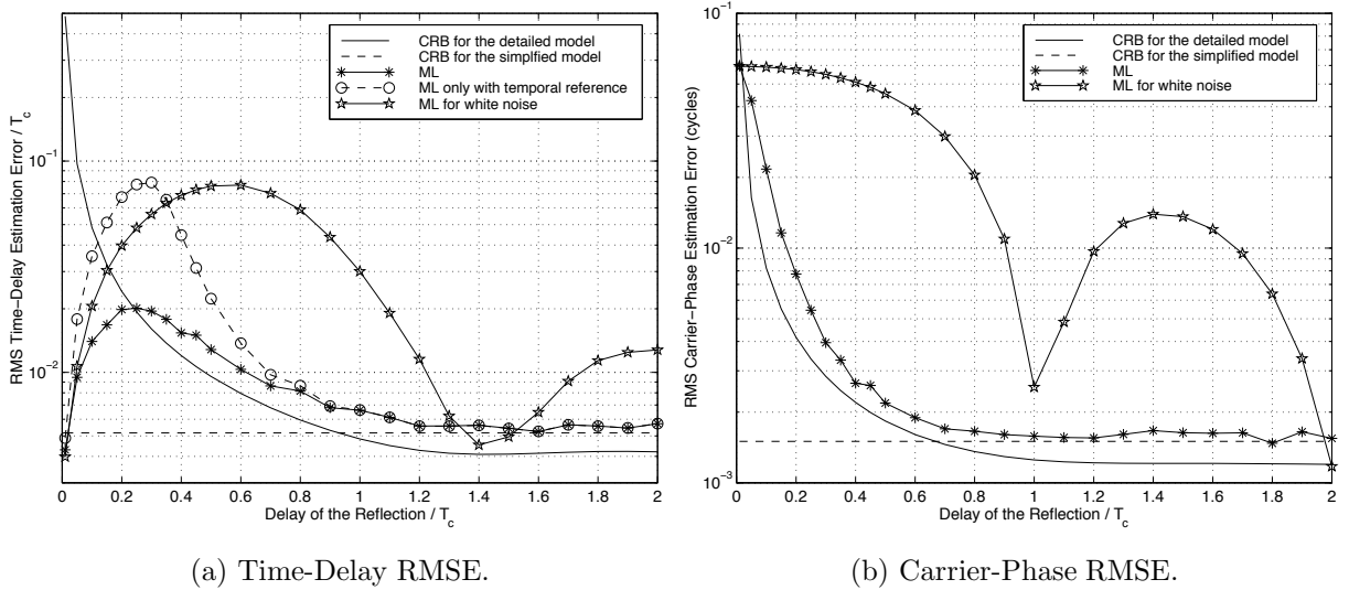
Figure 4.10: RMSE as a function of the delay of the reflection with respect to the direct signal. Parameters: \check{\theta}_0 = 0^\circ , \check{\tau}_0 = 0 , \check{\theta}_1 = 10^\circ , \check{\alpha}_0/\check{\alpha}_1 = \sqrt{2} , M = 3 pulses, m = 6 antennas, \text{SNR}_0 = 15.87 dB.
