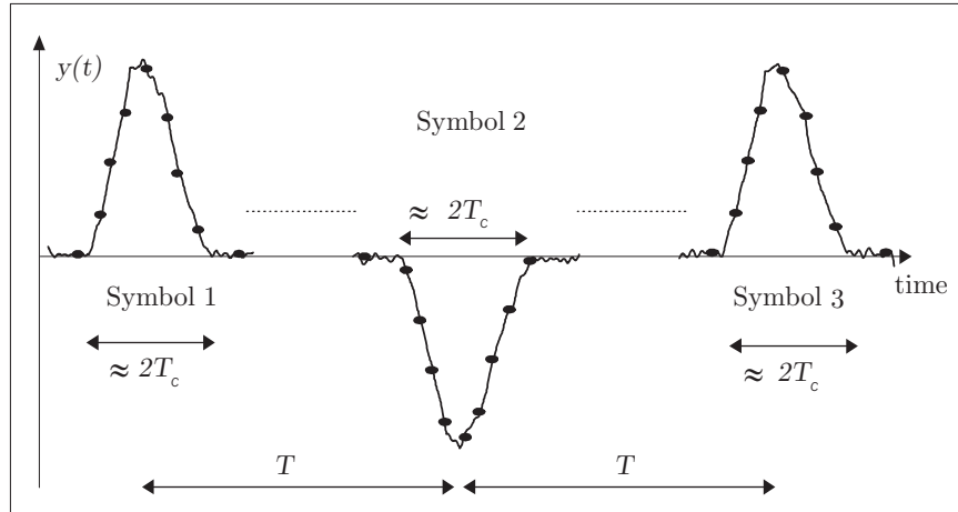
Figure 2.2: Qualitative example of the despread signals.
