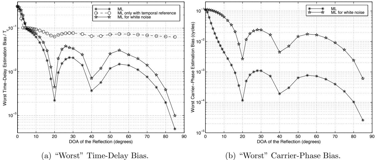
Figure 4.13: Dependence of the bias on the angular separation between the reflection and the direct signal. Parameters: \check{\theta}_0 = 0^\circ , \check{\tau}_0 = 0 , \check{\tau}_1 = 0.25T_c , |\check{\alpha}_0|/|\check{\alpha}_1| = \sqrt{2} , M = \infty pulses, m = 6 antennas, \text{SNR}_0 = 15.87 dB.
