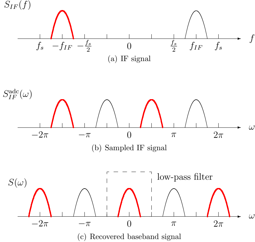
Figure 2.3: Representation of the spectral densities with f_{IF} = 3f_s/4 : (a) x_{IF}(t) , (b) x_{IF}[n] and (c) x[n] = x_{IF}[n] \cdot e^{-j\frac{\pi}{2}n} .
