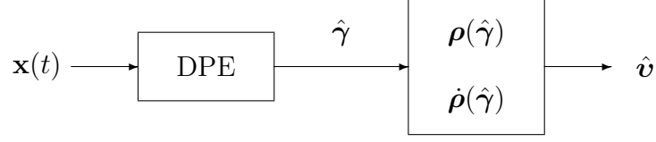
Figure 4.10: Position-based Synchronization. Time-delays and Doppler-shifts can be obtained from DPE solution.
