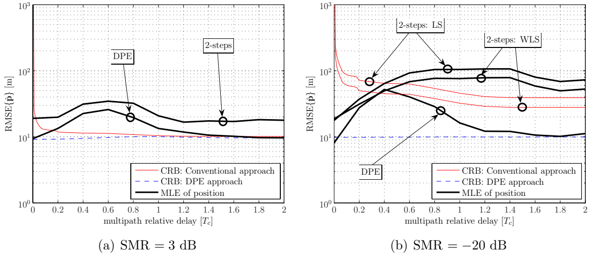
Figure 4.12: \text{RMSE}\{\hat{\mathbf{p}}\} of MLE of position against CRBs as a function of the relative multipath delay. Scenario 3 in (a) and Scenario 4 in (b), with N = 1 antenna.
