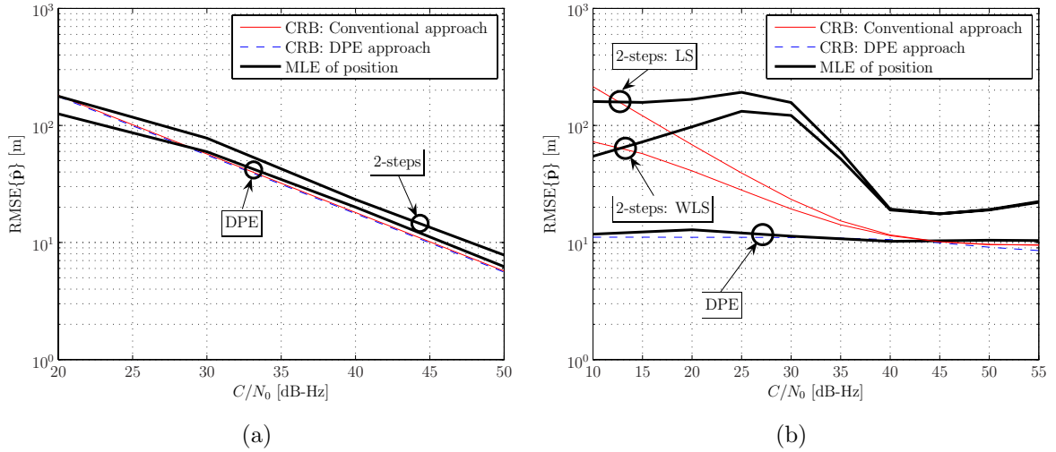
Figure 4.11: \text{RMSE}\{\hat{\mathbf{p}}\} of MLE of position against the corresponding CRB. Scenario 1 in (a) and Scenario 2 in (b), with N = 1 antenna.
