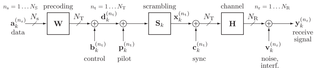
Figure 3.1: Generalized system model of the HSDPA physical layer.
