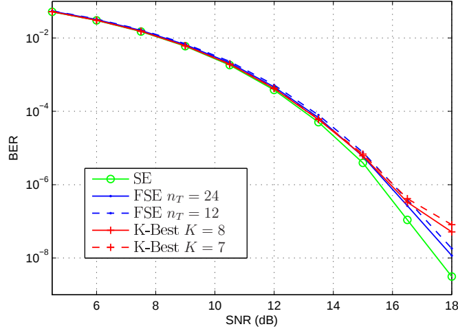
Figure 4.13: BER performance of the SE, the FSE with n_T = 12 and n_T = 24 and the K-Best with K = 7 and K = 8 in an 8 \times 8 VP system.
