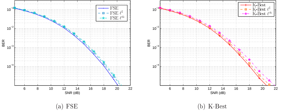
Figure 6.7: BER performance degradation introduced by approximating the \ell^2 norm by the simplified \ell^1 and \ell^\infty norms in the FSE ( n_T = 10 ) (a) and K-Best ( K = 7 ) (b) tree-search approaches.
