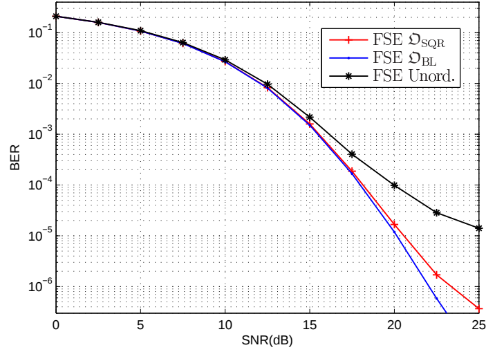
Figure 4.6: BER performance of the proposed FSE algorithm with \mathbf{n} = [1, 1, 2, 5] and ordering strategies \mathcal{D}_{\text{SQR}} and \mathcal{D}_{\text{BL}} . Additionally, the unordered case is included for completion.
