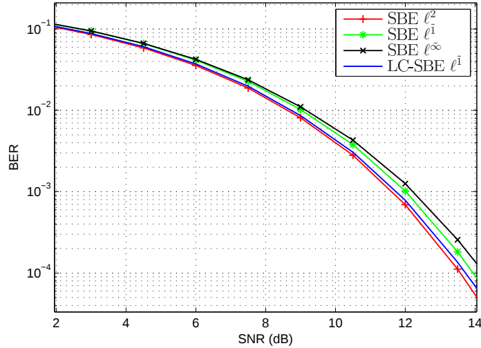
Figure 7.5: BER performance of the LC-SBE and the SBE algorithm with the \ell^2, \ell^1 and \ell^\infty approaches for distance computation.
