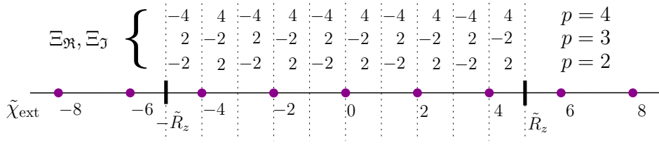
Figure 5.12: Values of the \Xi_{\Re} and \Xi_{\Im} increments for different regions of the \tilde{\chi}_{\text{ext}} axis for the 2 nd , 3 rd and 4 th closest nodes in the real axis.
