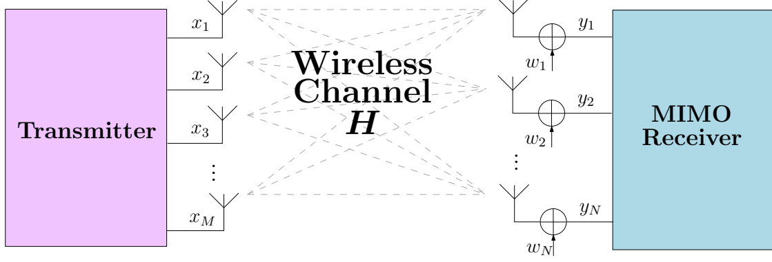
Figure 2.1: Block diagram of an N \times M MIMO system where M stands for the number of transmit antennas and N represents the number of receive antennas.
