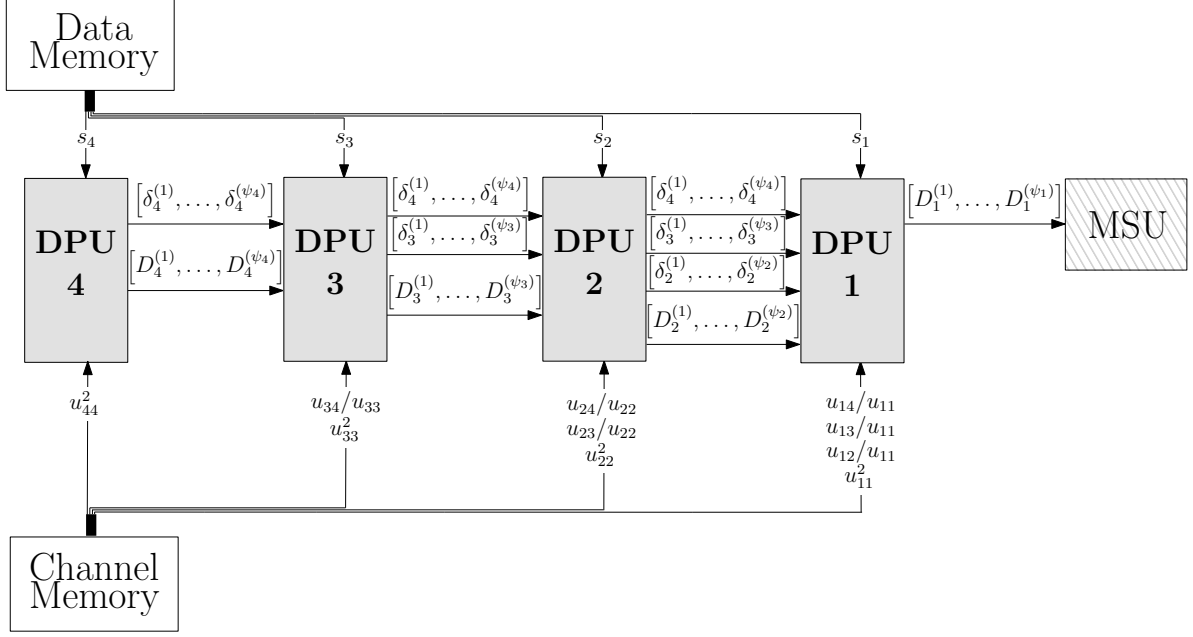
Figure 6.1: General hardware architecture of the fixed-complexity tree-search techniques for an N = 4 user system.
