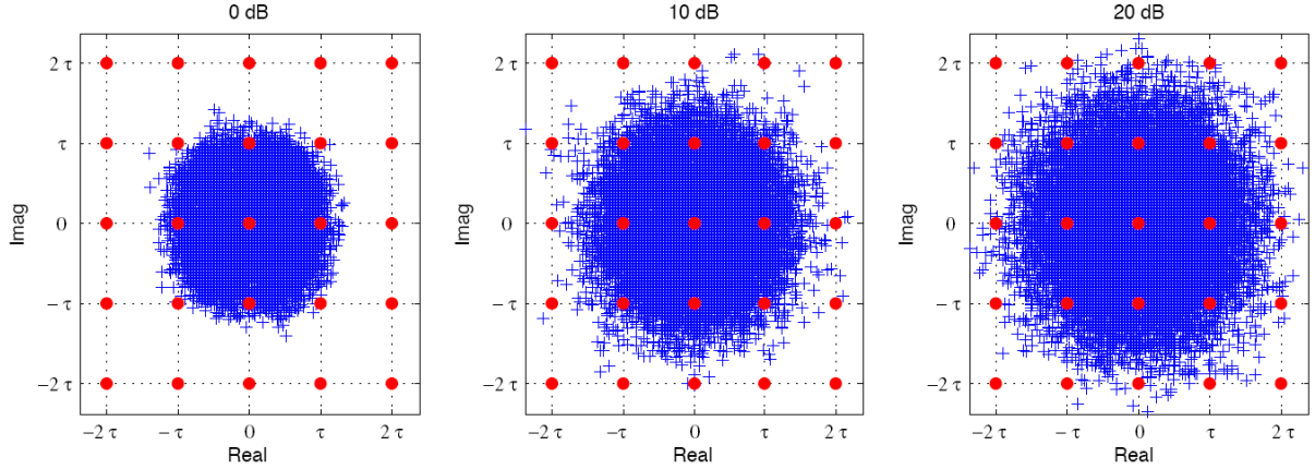
Figure 5.6: Distribution of the intermediate points for several SNR values.
