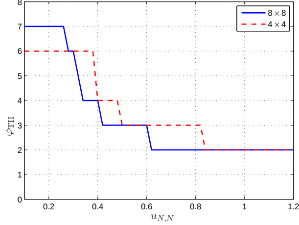
Figure 7.7: Run-time constraint values ( \varphi_{TH} ) for 4 \times 4 and 8 \times 8 antenna setups with p = 0.9 .
